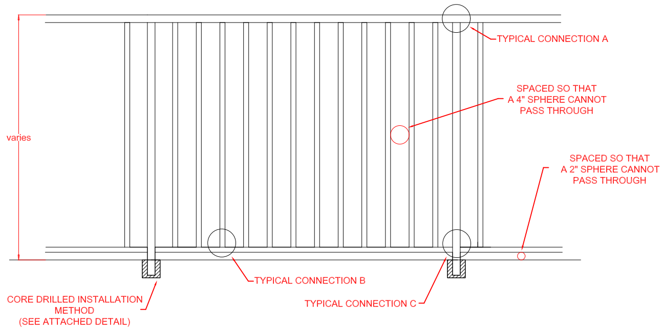
STANDARD GUARDRAIL
